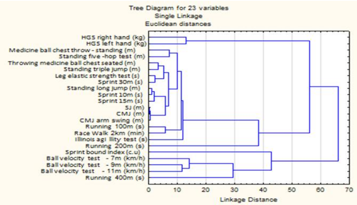
Figure 1. Cluster analysis
